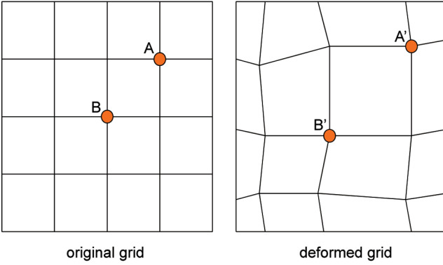
Fig. 3. The deformed grid records how the reduced data set is deformed. Specifically, in this example, the voxels A and B are stored in the positions of A' and B' , respectively. The only additional computation of rendering is a texture lookup to figure out where the voxel is stored.
